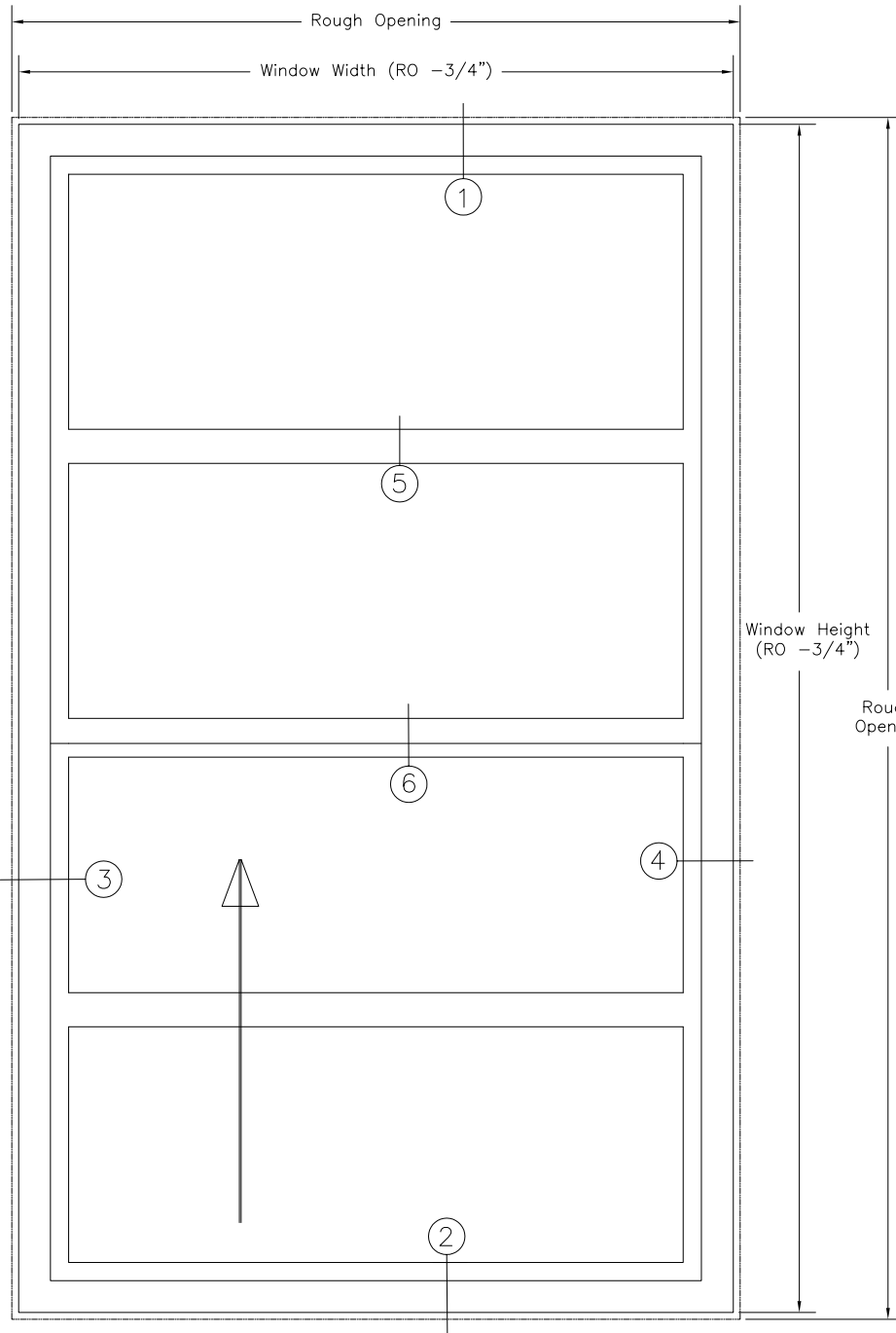
Fyre-Tec Series 925 Single Hung 45 Or 60 Minute UL Rated Typical Exterior Elevation (Muntins Required on Larger Sizes with Wire Glass. Optional with 60 Minute Glazing)
