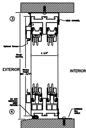
Prime-Tec Series 300 - 400 Horizontal Slider Typical Head/Sill Section
