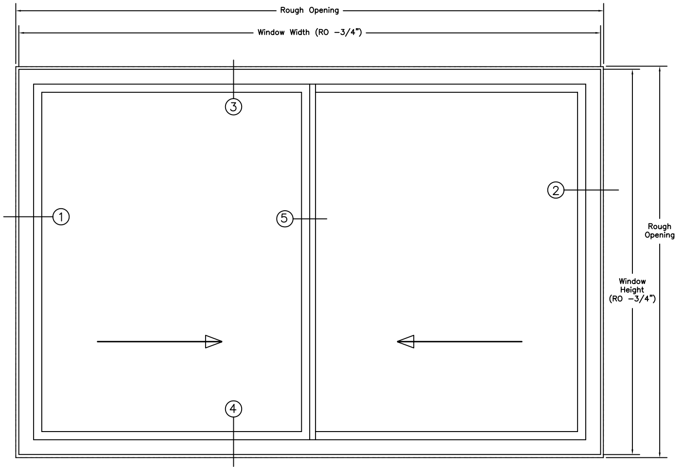
Prime-Tec Series 400 Horizontal Slider Single Slide Series 300 Available Typical Exterior Elevation (Muntin Configuration and Glazing Type Optional)
