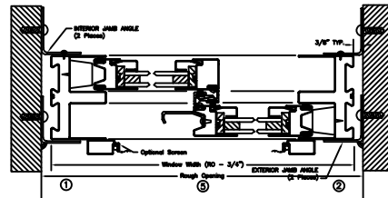
Prime-Tec Series 300 - 400 Horizontal Slider Typical Jamb Section
